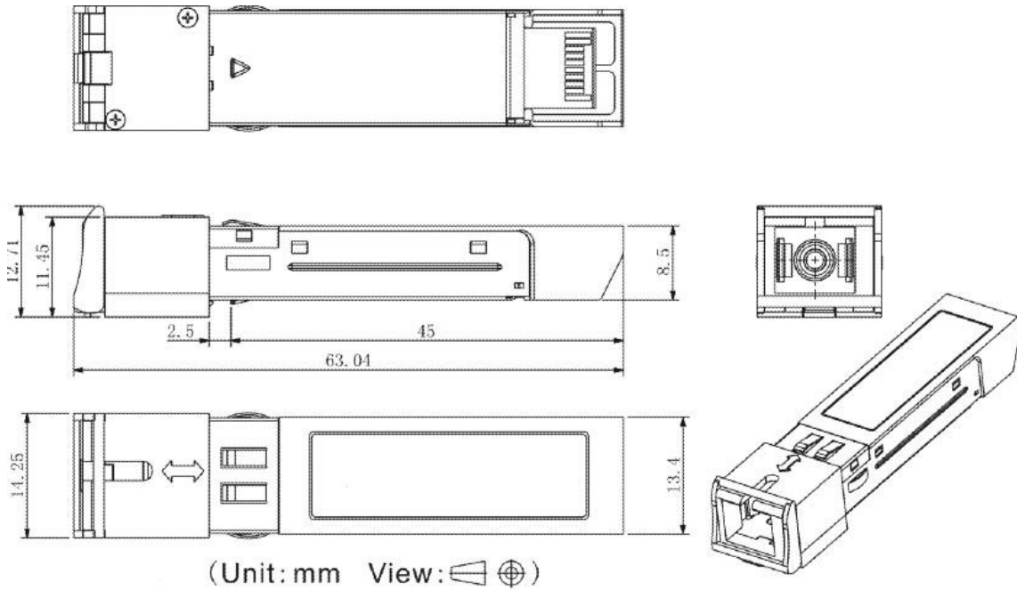
Mechanical Drawing
