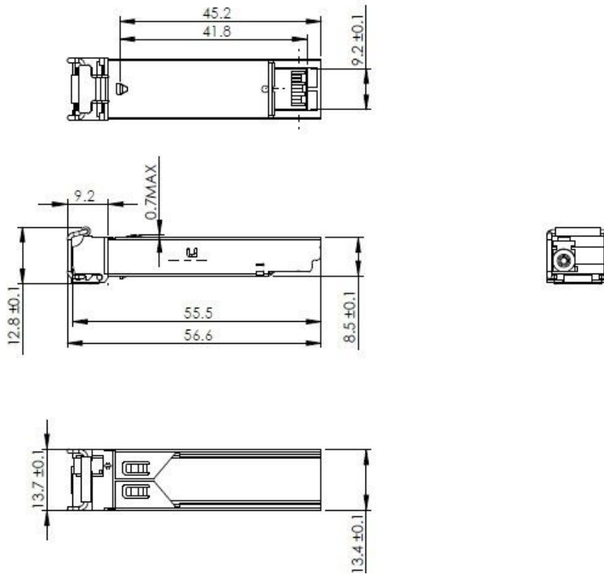
Mechanical Drawing
