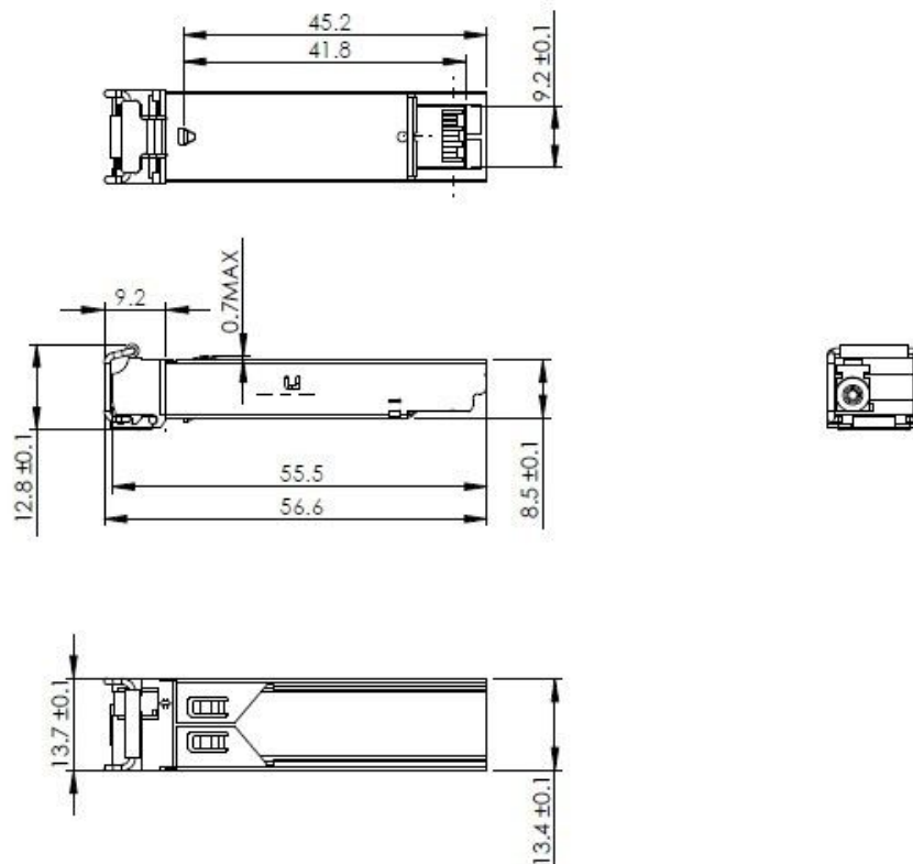
Mechanical Drawing
