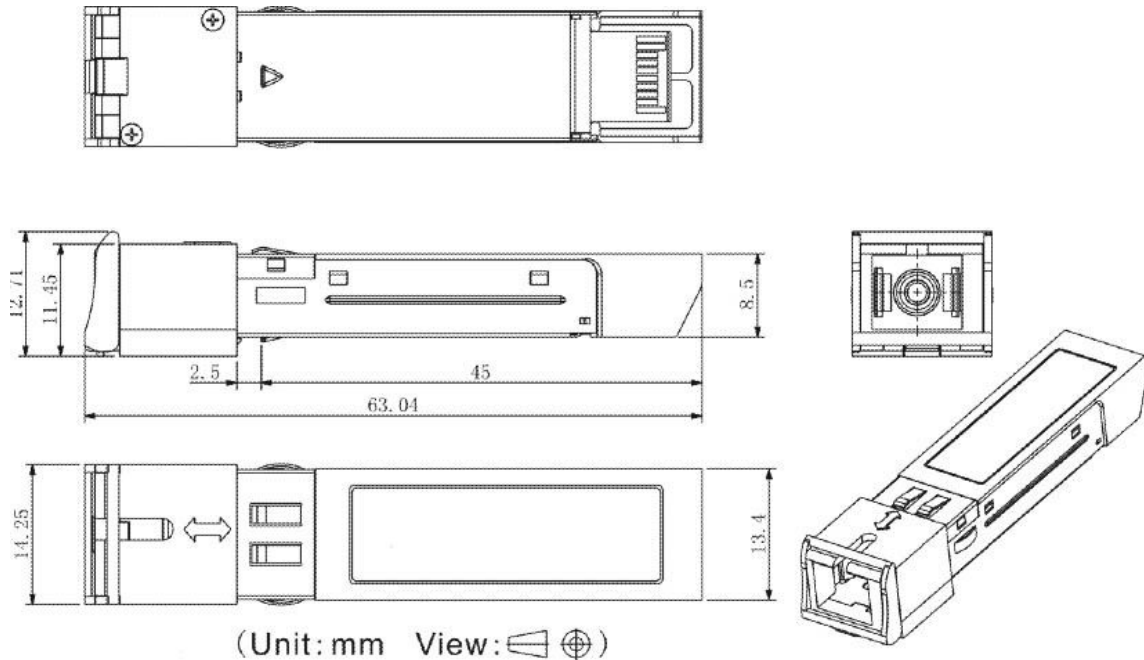
Mechanical Drawing
