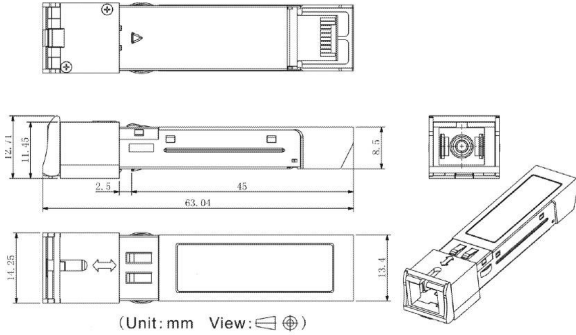
Mechanical Drawing
