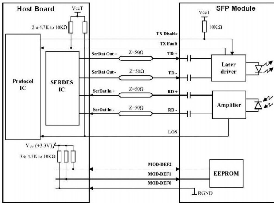
SFP Host Recommended Circuit
