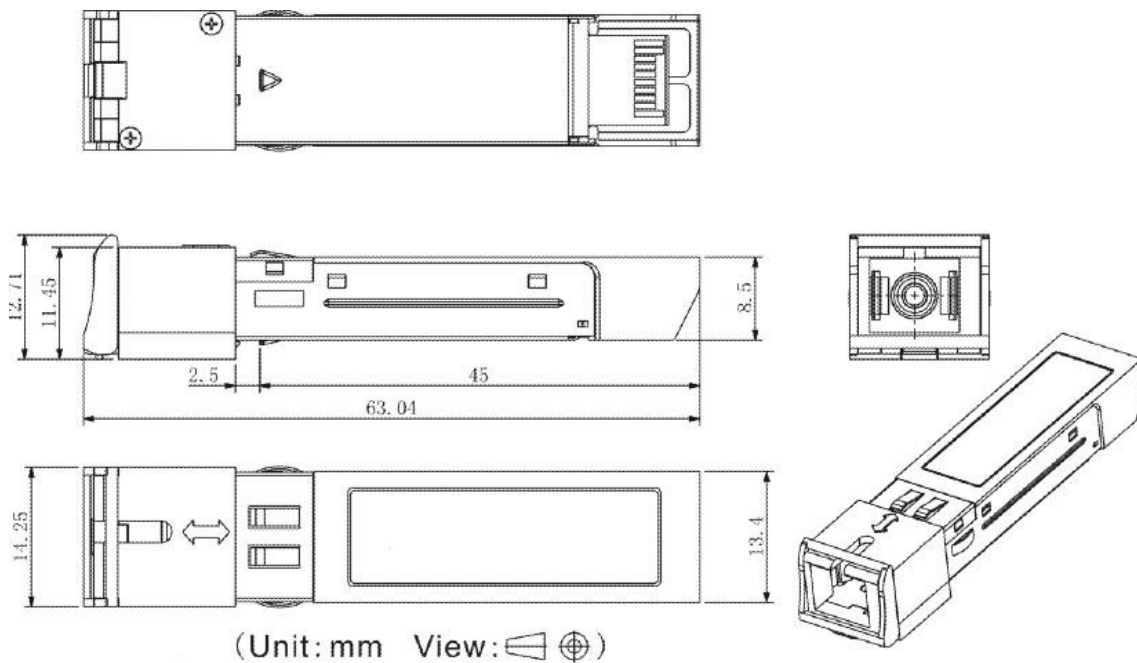
Mechanical Drawing
