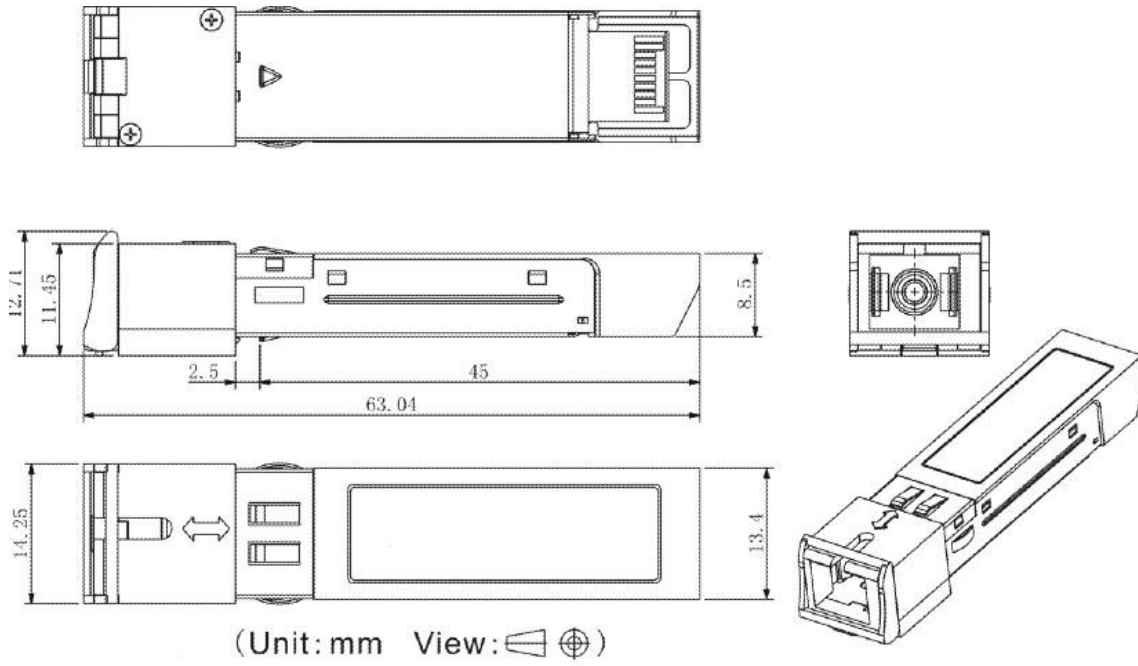
Mechanical Drawing
